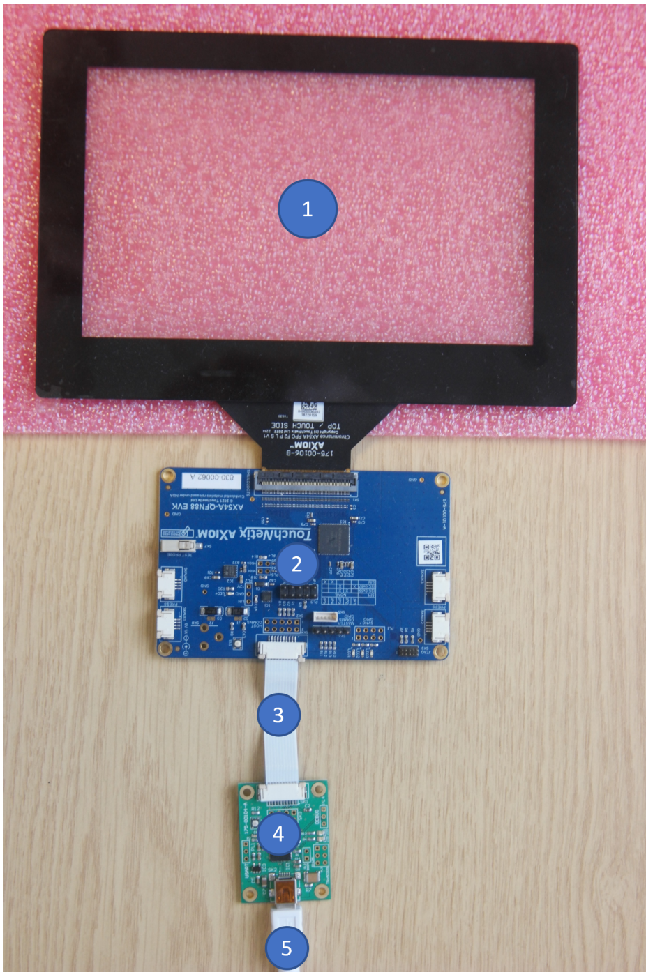
Figure 3-1: AX54A EVK Connection Image
